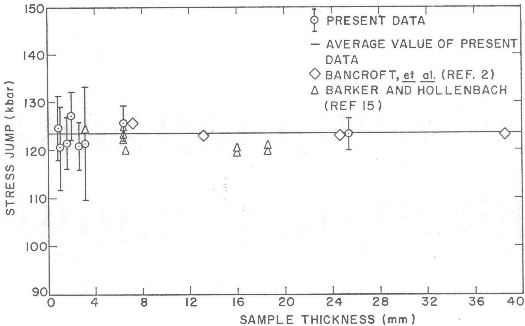
Fig. 4.4.--Stress jump across the plastic I shock as a function of sample thickness.
